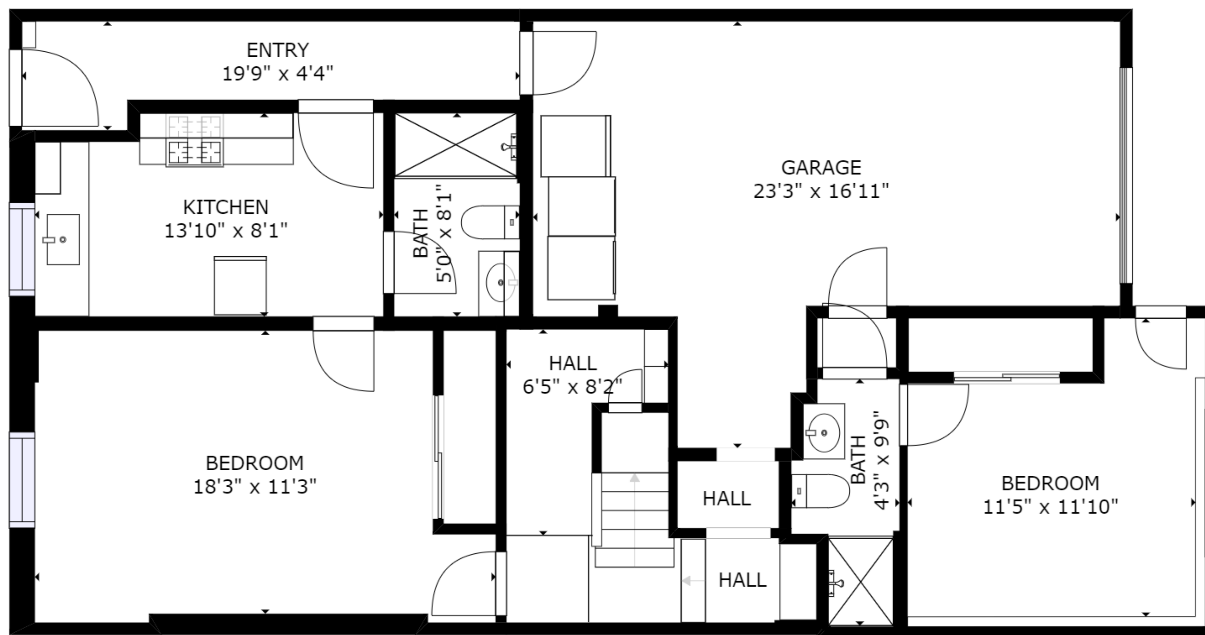
FLOOR 1
