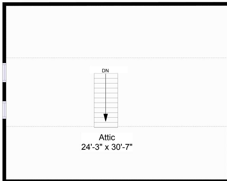
Attic Plan Ceiling Height = 7'-11"
