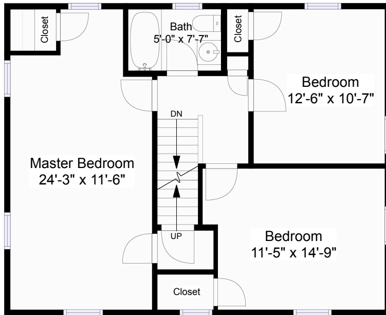
Second Floor Plan Ceiling Height = 7'-6"
