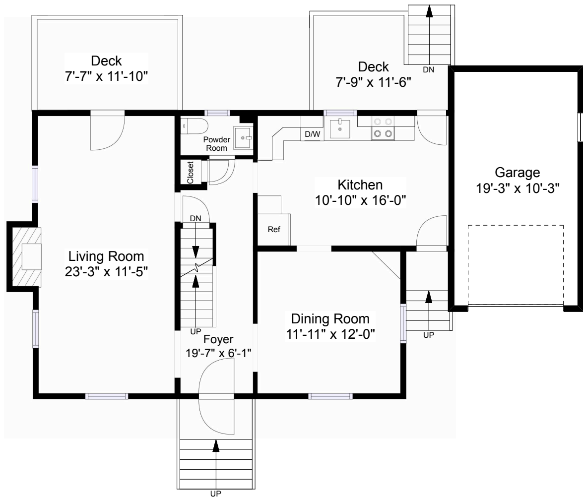
First Floor Plan Ceiling Height = 7'-8"
