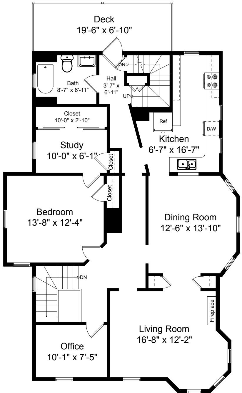
Second Floor Plan Ceiling Height = 9'-0"
