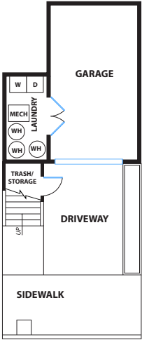
LOWER LEVEL
