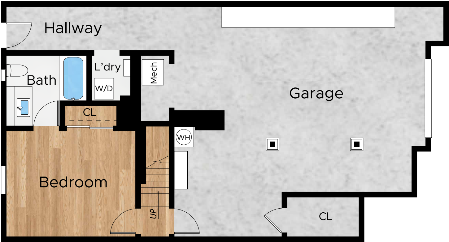
First Floor
