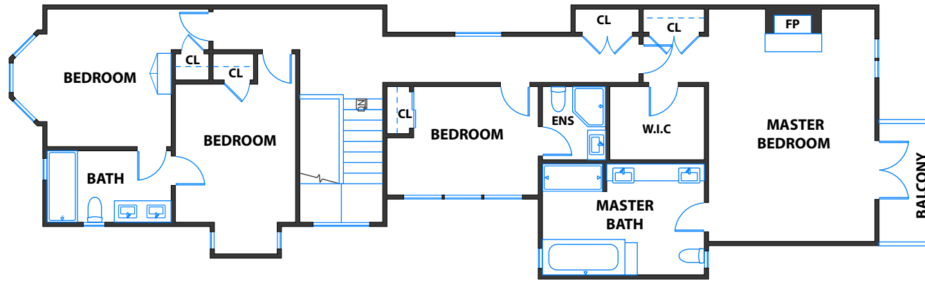
THIRD LEVEL
