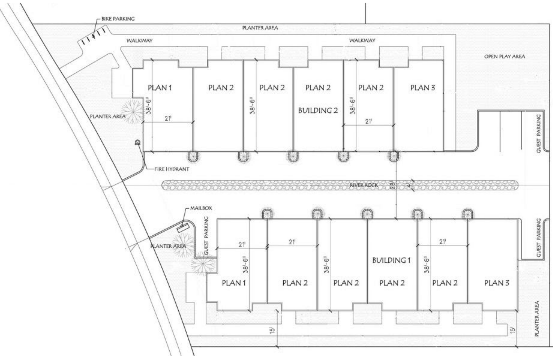
Site Plan - Lower Level & Garage
