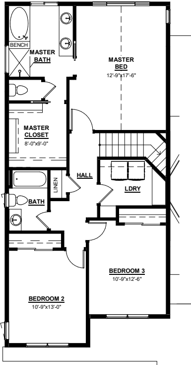
SECOND LEVEL FLOOR PLAN 1020 SF
