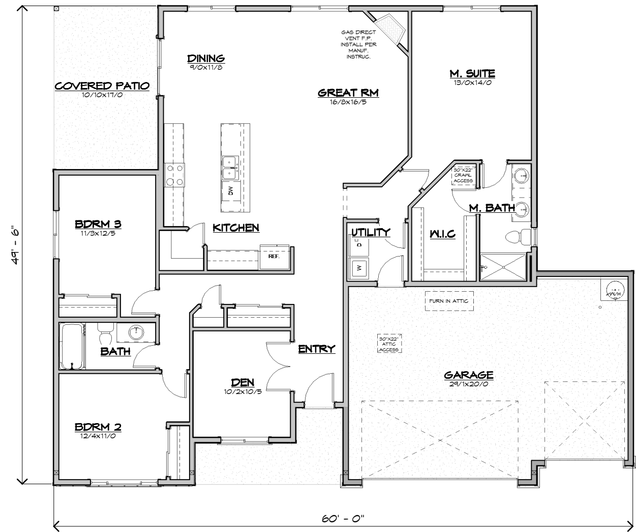
Main Floor Plan - 1800 SF
