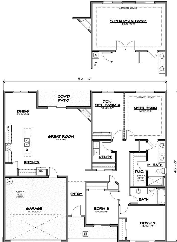
Main Floor Plan - 1902 SF
