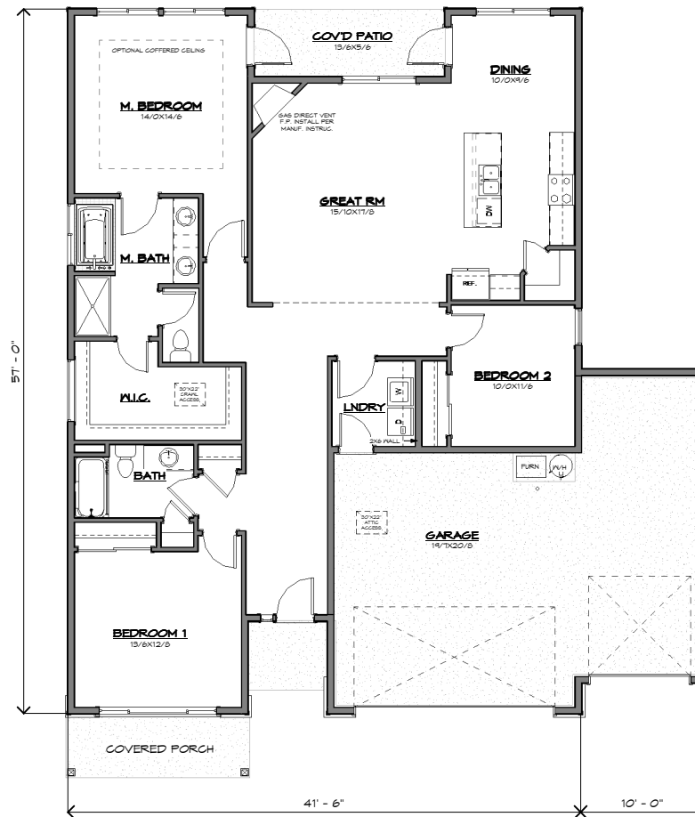
Main Floor Plan - 1798 SF
