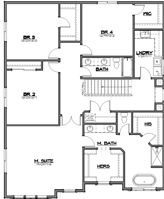
Upper Floor Plan- 1850 SF
