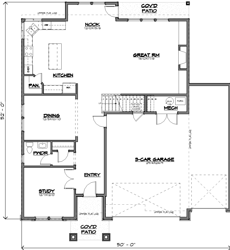
Main Floor Plan - 1387 SF
