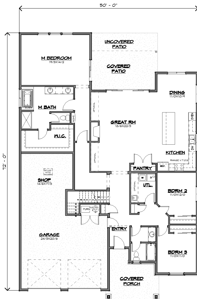
Main Floor Plan - 2237 SF
