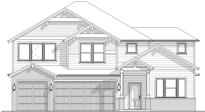
FRONT ELEVATION "A"
