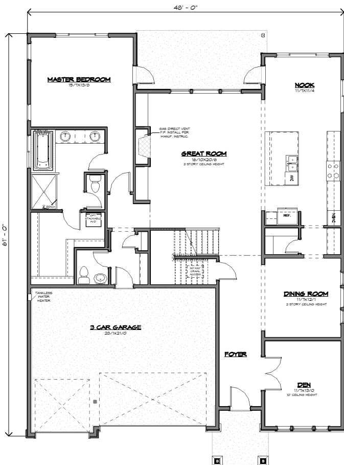
Main Floor Plan - 2046 SF
