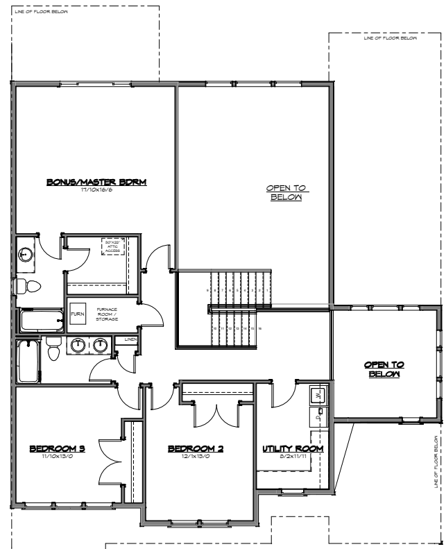
Upper Floor Plan - 1251 SF
