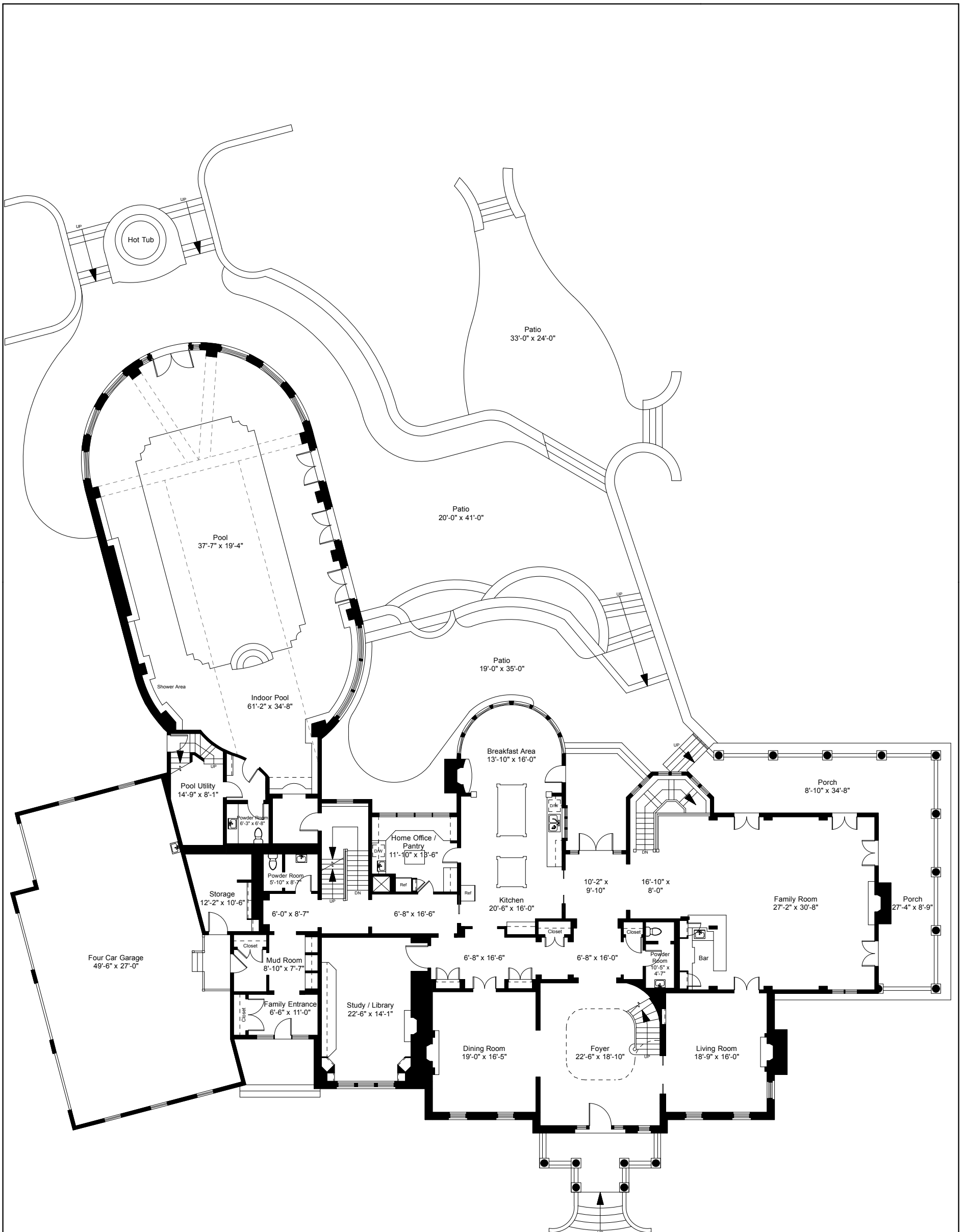
First Floor Plan Ceiling Height = 11'-2"
